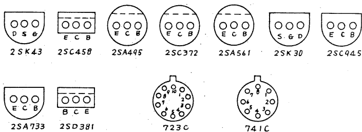
Fig. 5-3 Pins of transistors and IC's (bottom view)
